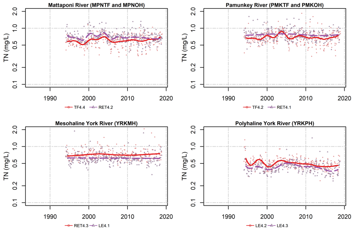
Figure 7. Surface TN data (dots) and average long-term pattern generated from non-flow adjusted GAMs. Colored dots represent data corresponding to the monitoring station shown indicated in the legend; colored lines represent mean annual GAM estimates for the noted monitoring stations.
