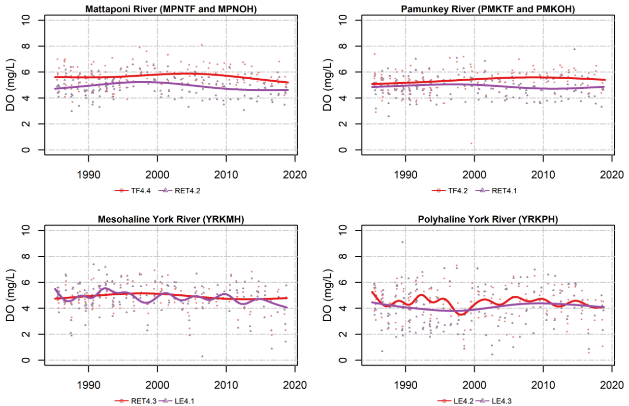
Figure 17. Summer (June-September) bottom DO data (dots) and mean summer long-term pattern generated from non-flow adjusted GAM. Colored dots represent June-September data corresponding to the monitoring station indicated in the legend; colored lines represent mean summer GAM estimates for the noted monitoring stations.
