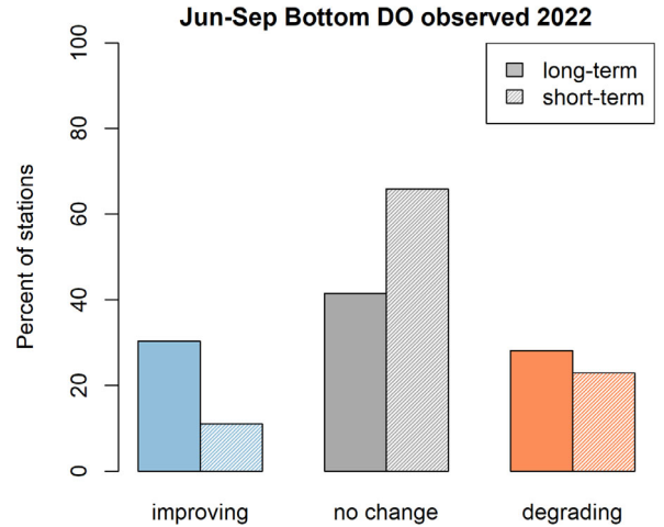
Figure 1. Percent of stations with improving, degrading, and no change for dissolved oxygen in the bottom layer during the summer season for long- and short-term periods.
