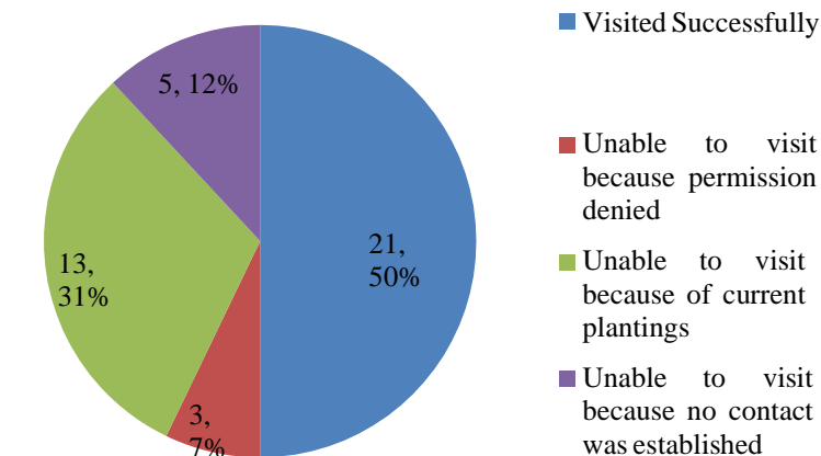
Figure 2: Pie Graph showing successful site visits
