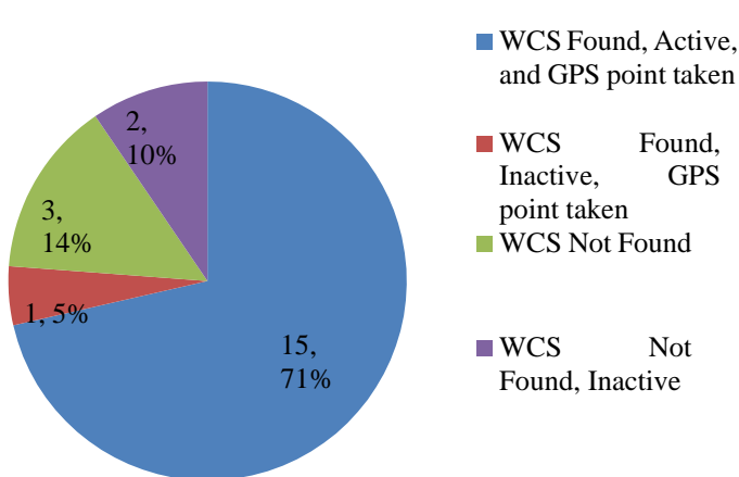
Figure 1: Pie Graph showing successful data point collection
