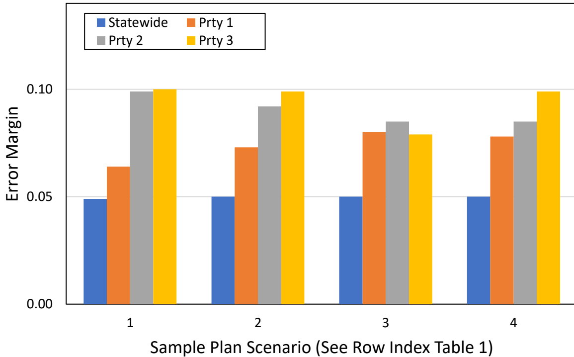
Figure 1. Summary of error margin calculations by sampling scenario
